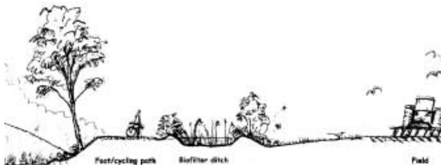
Principal section of the Vagnhärad pond system
